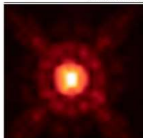
Artist's conception of images made by NASA's Hubble and Spitzer telescopes.
